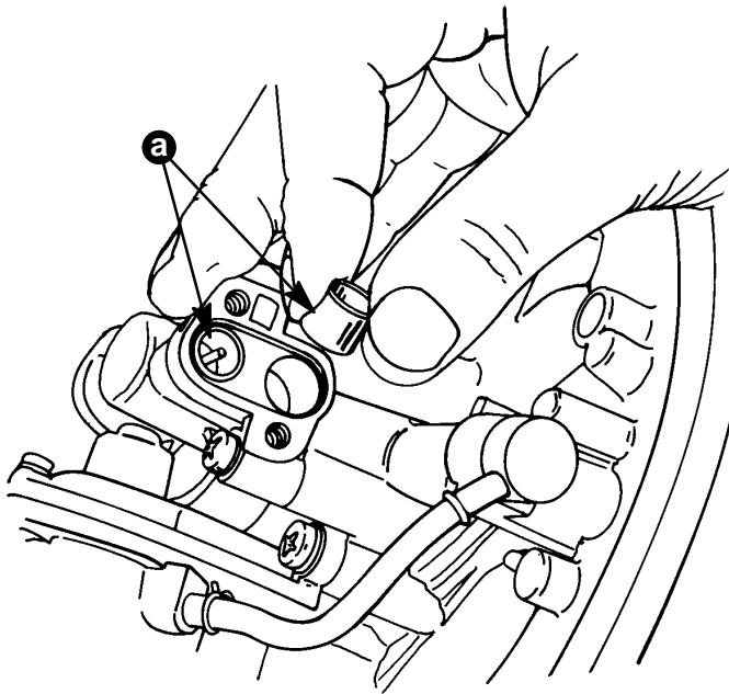
Figure 1. Bottom View of AutoBlend with Oil Pickup Tube Removed
