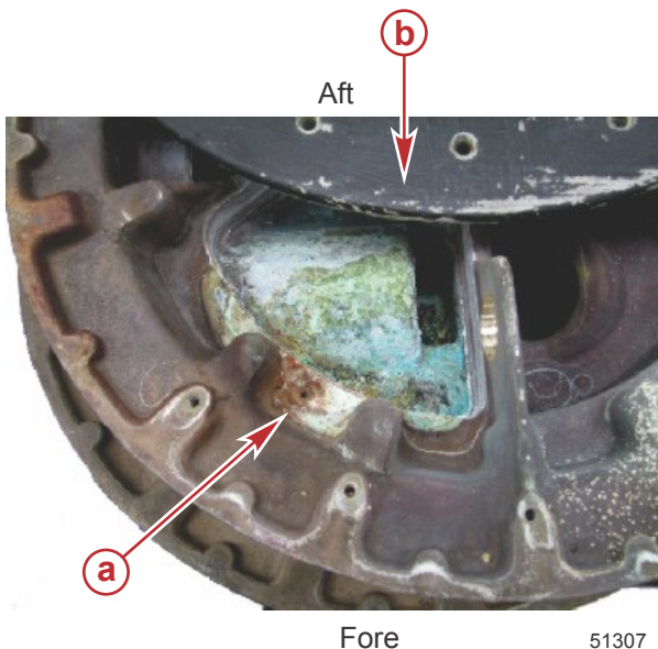
View from below with the seawater intake cover removed
