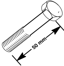
Puller Bolt P/N 10-40001149
