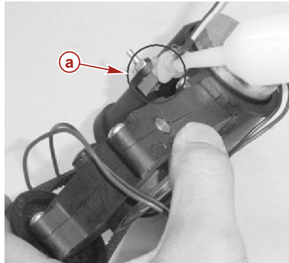
a - Apply Dielectric Grease under the potentiometer switch
